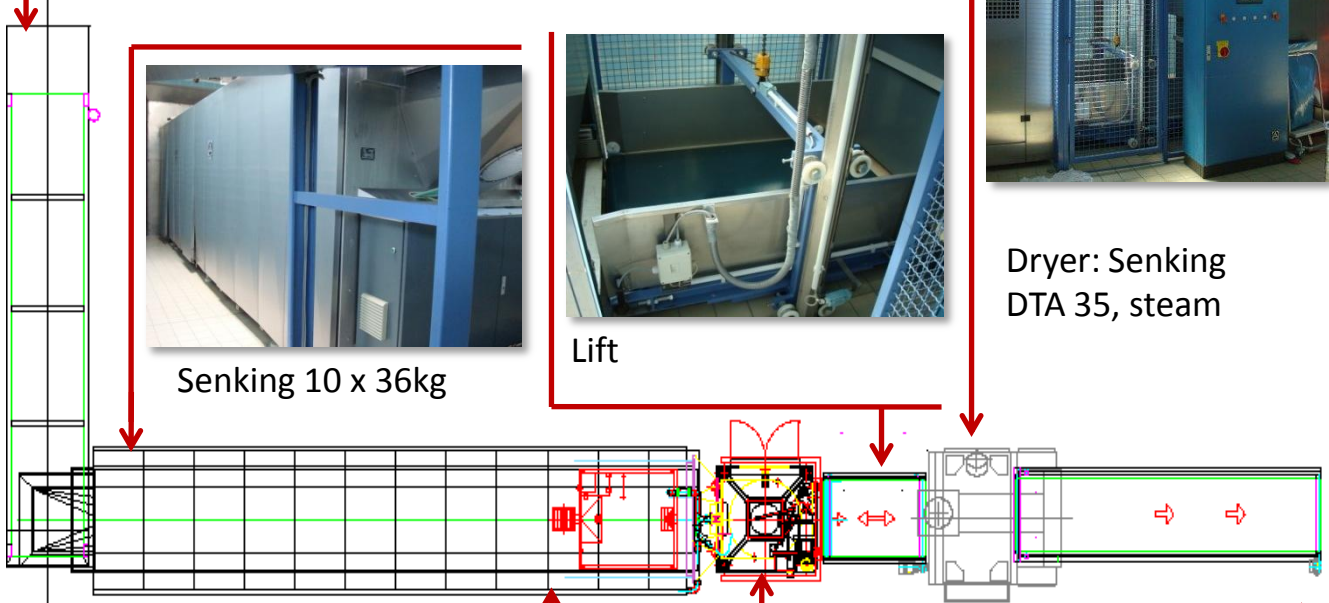
Step conveyor With integrated Weighing system
